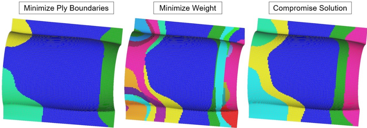
Figure 4. HyperSizer zone shapes for a turbofan Inner Fixed Structure (IFS). [1]
