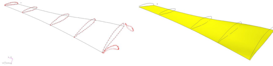
Figure 3. (a) Measured points (b) Closed loop cross-sections and surface.
