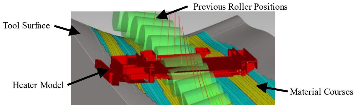
Figure 7. Heater orientation optimization.
