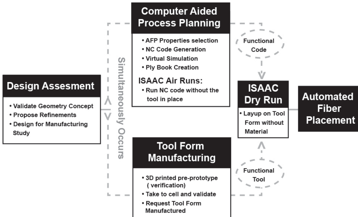
Figure 6. Manufacturing flowchart.
