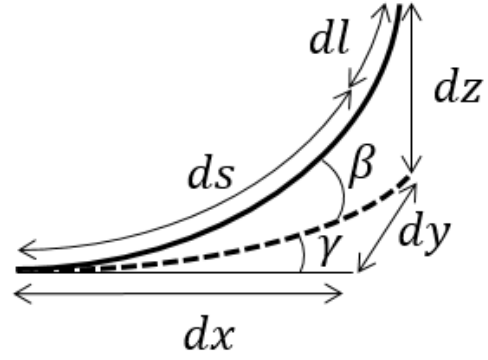
Figure 5. Strain rotation relationship in 3D
