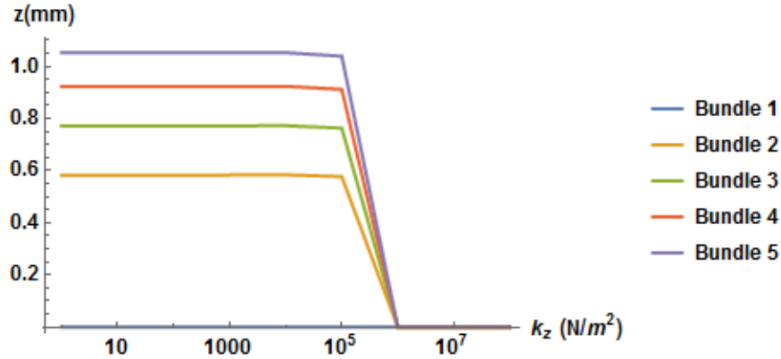
Figure 11: Effect of the foundation stiffness in the z -direction on the wrinkle formation
