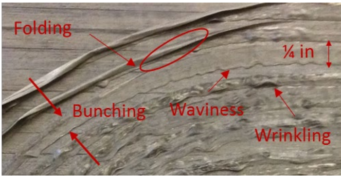
Figure 2. Tow deformations due to excessive steering (Courtesy of McNair Center, University of South Carolina) [6]
