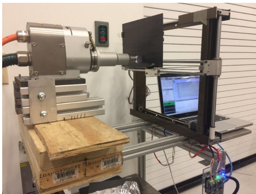
Figure 1 Atmospheric pressure plasma jet treatment system
