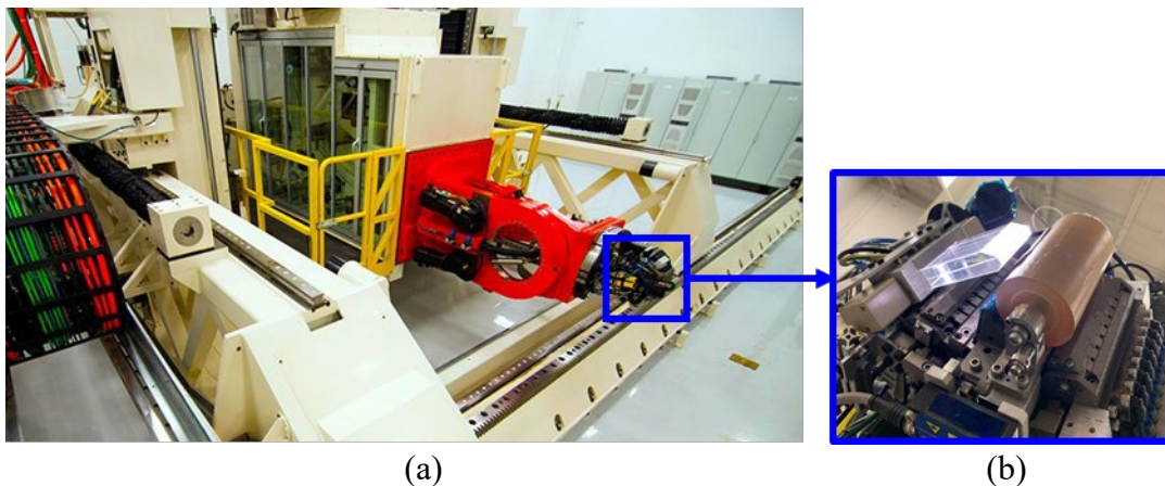
Figure 1: Image of the AFP machine and fiber placement head
