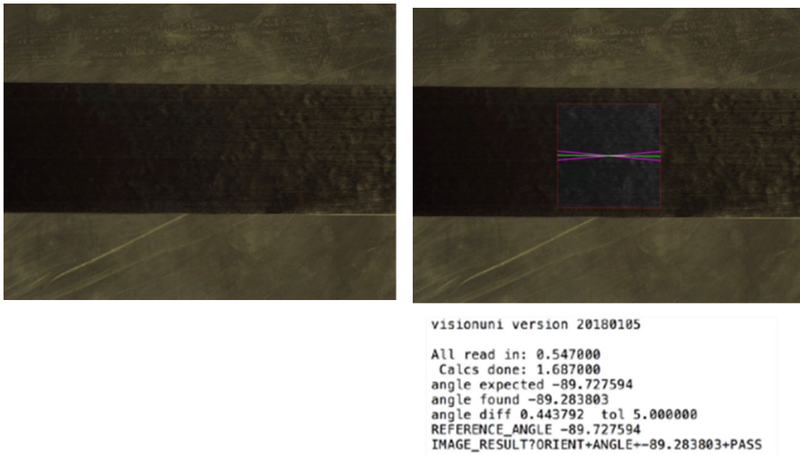
Figure 4. Raw (left) and analyzed (right) image from large-field automatic inspection system verifying that fiber orientation is within tolerance.
