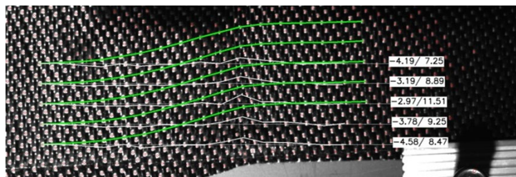
Figure 9. Automatic discovery of fiber paths in material sheared in press
