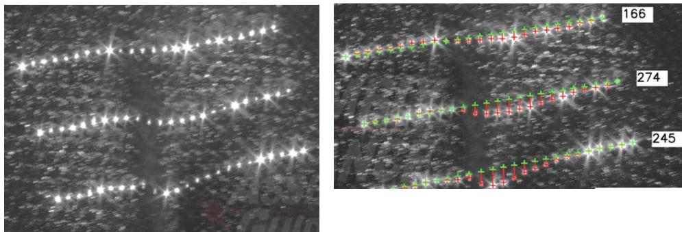
Figure 7. Automatic detection of 0.8mm wrinkle in robotic layup system
